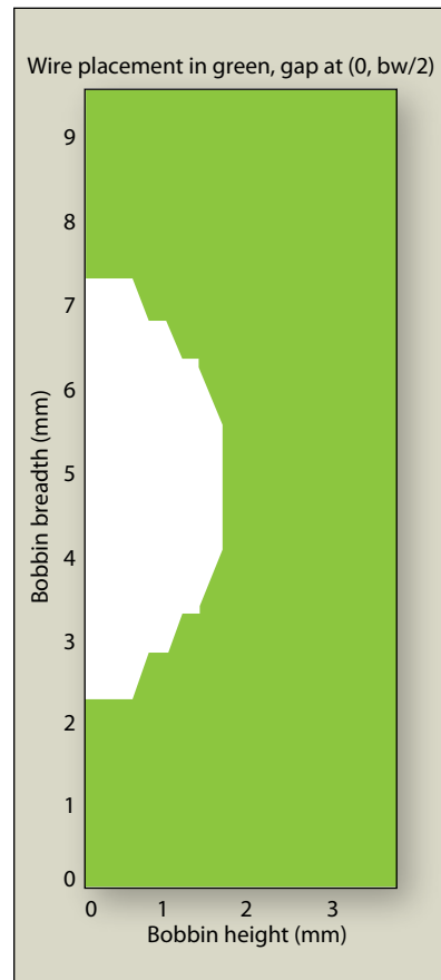
Fig. 3. The ShapeOpt program determines the optimal placement of the winding inside the specified bobbin window for a 10.6- \mu H inductor.
